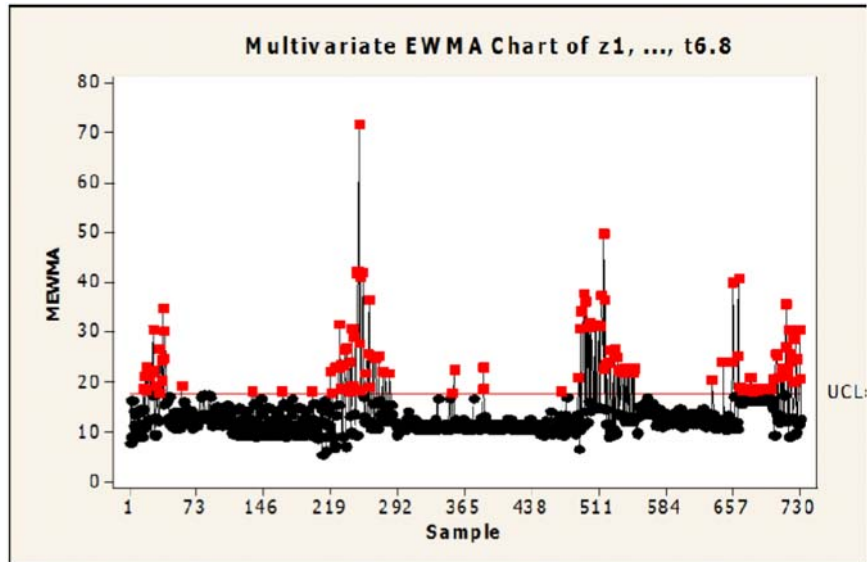
Figure 22. MEWMA chart of Z_1, \dots, t_{6.8} with ARL = 100 , r = 0.5 .
