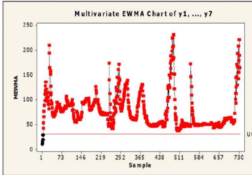
Figure 6. MEWMA chart of y_1, \dots, y_7 with ARL = 200 , r = 0.1 .
