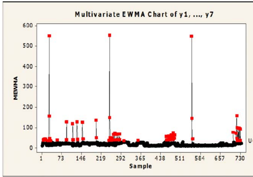
Figure 21. MEWMA chart of y_1, \dots, y_7 with ARL = 400 , r = 0.5 .
