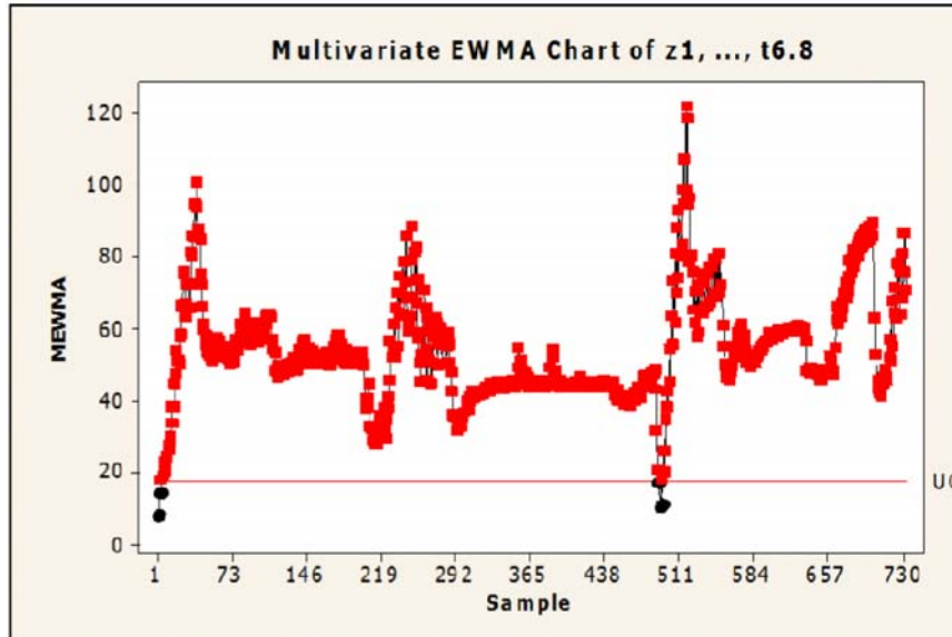
Figure 11. MEWMA chart of Z_1, \dots, t_{6.8} with ARL = 200 , r = 0.1 .
