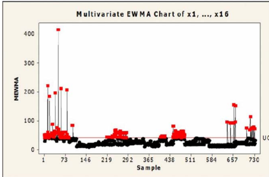
Figure 4. MEWMA chart of X_1, \dots, X_{16} with ARL = 200 , r = 0.7 .
