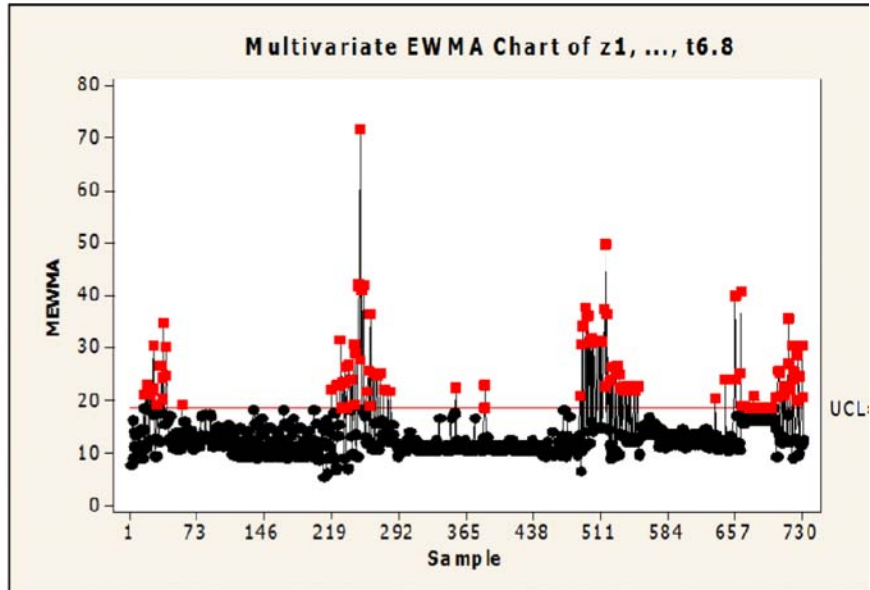
Figure 13. MEWMA chart of Z_1, \dots, t_{6.8} with ARL = 200 , r = 0.5 .
