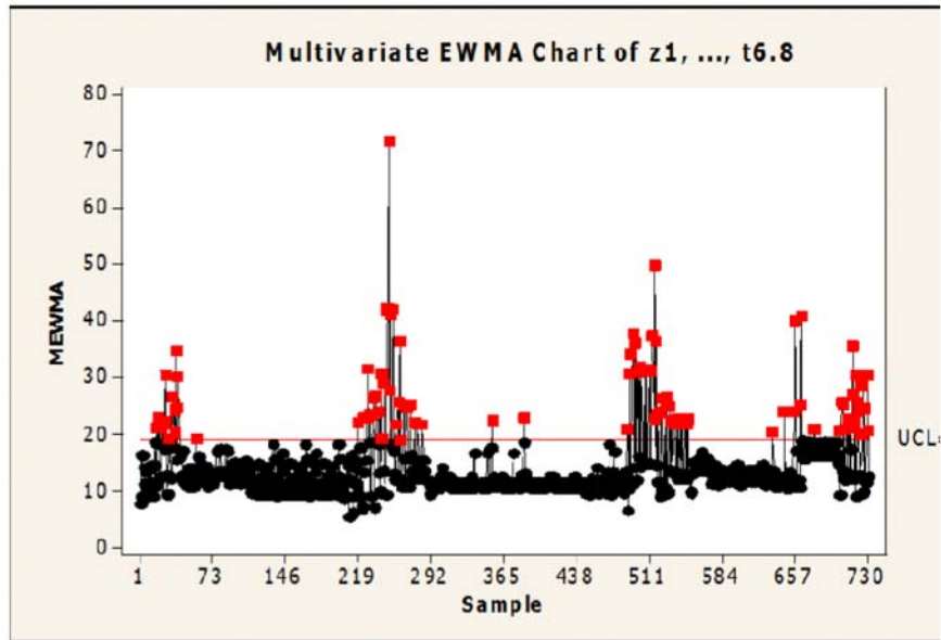
Figure 23. MEWMA chart of Z_1, \dots, t_{6.8} with ARL = 300 , r = 0.5 .
