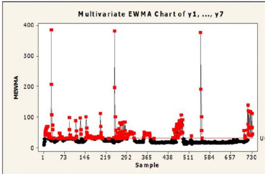
Figure 7. MEWMA chart of y_1, \dots, y_7 with ARL = 200 , r = 0.3 .
