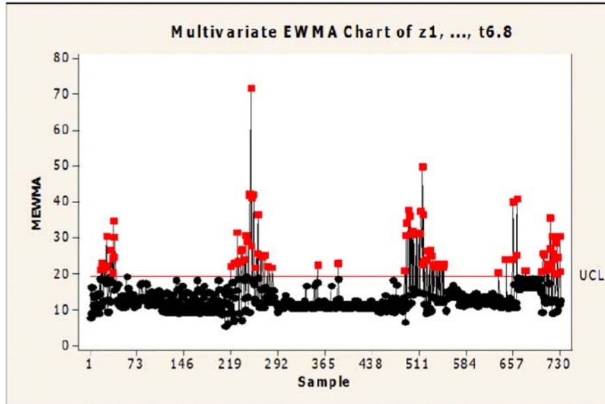
Figure 24. MEWMA chart of Z_1, \dots, t_{6.8} with ARL = 400 , r = 0.5 .
