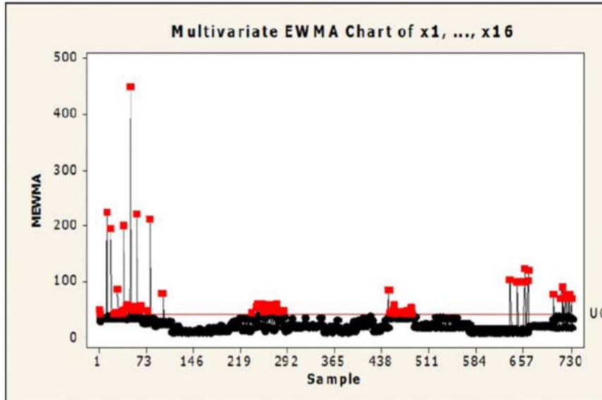
Figure 5. MEWMA chart of X_1, \dots, X_{16} with ARL = 200 , r = 0.9 .
