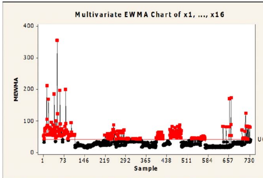
Figure 17. MEWMA chart of X_1, \dots, X_{16} with ARL = 300 , r = 0.5 .
