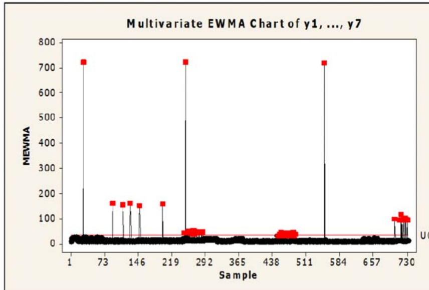
Figure 10. MEWMA chart of y_1, \dots, y_7 with ARL = 200 , r = 0.9 .
