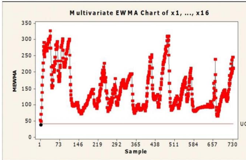
Figure 1. MEWMA chart of X_1, \dots, X_{16} with ARL = 200 , r = 0.1 .
