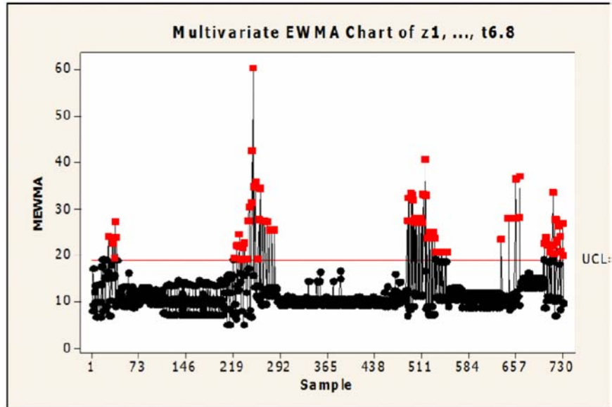
Figure 14. MEWMA chart of Z_1, \dots, t_{6.8} with ARL = 200 , r = 0.7 .
