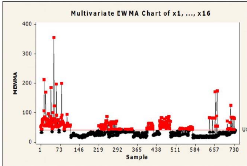
Figure 3. MEWMA chart of X_1, \dots, X_{16} with ARL = 200 , r = 0.5 .
