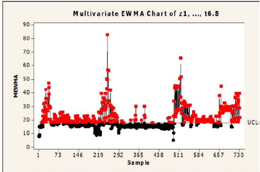
Figure 12. MEWMA chart of Z_1, \dots, t_{6.8} with ARL = 200 , r = 0.3 .
