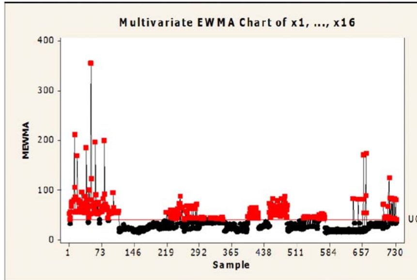
Figure 16. MEWMA chart of X_1, \dots, X_{16} with ARL = 100 , r = 0.5 .
