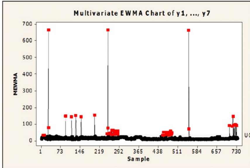
Figure 9. MEWMA chart of y_1, \dots, y_7 with ARL = 200 , r = 0.7 .
