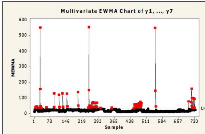
Figure 8. MEWMA chart of y_1, \dots, y_7 with ARL = 200 , r = 0.5 .
