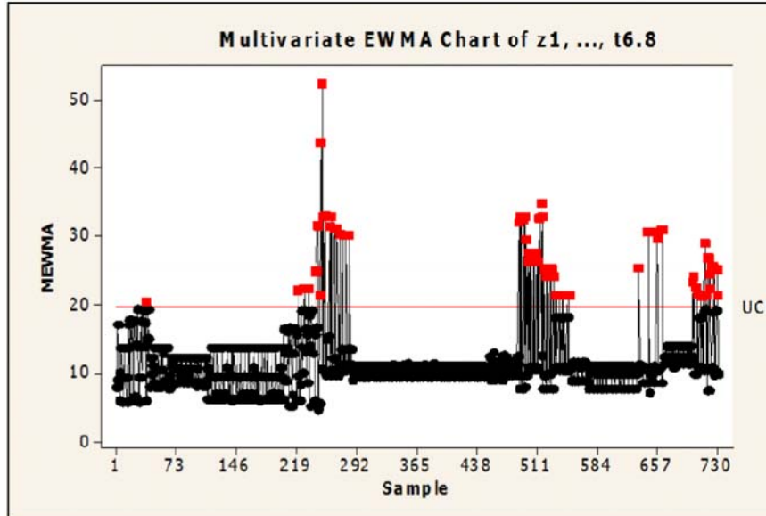
Figure 15. MEWMA chart of Z_1, \dots, t_{6.8} with ARL = 200 , r = 0.9 .
