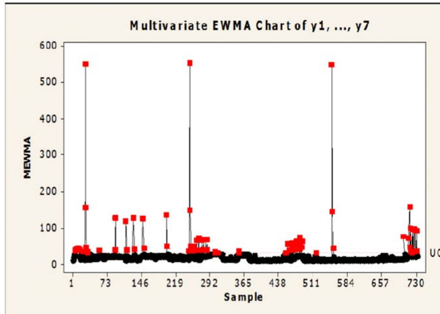
Figure 19. MEWMA chart of y_1, \dots, y_7 with ARL = 100 , r = 0.5 .
